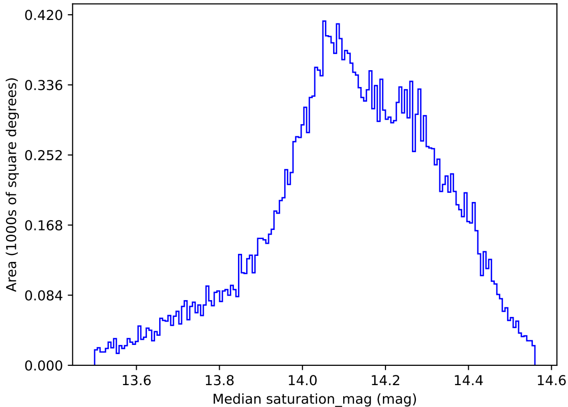
early_ss_template_fpextra2.0_v3.4_10yrs All sky all bands: Median saturation_mag
