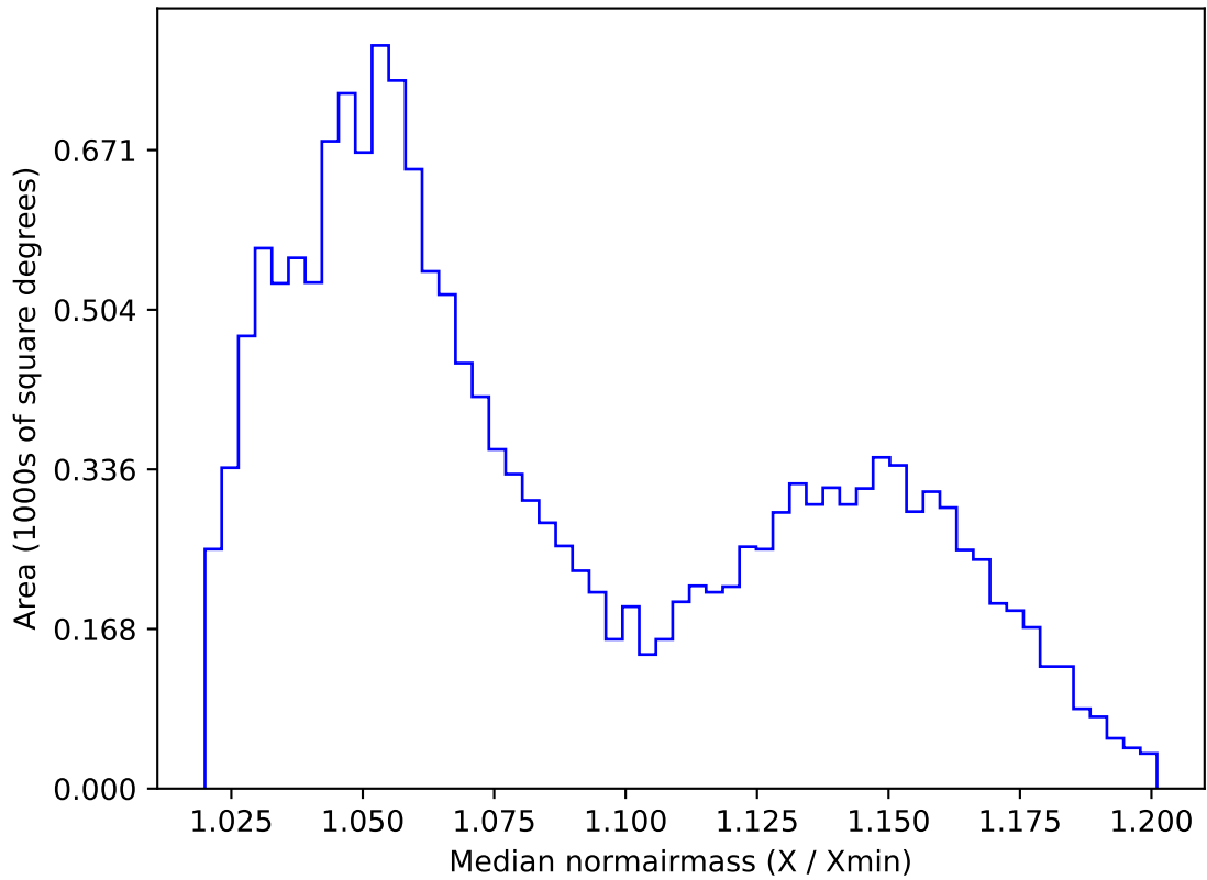
early_ss_template_fpextra2.0_v3.4_10yrs WFD z band: Median normairmass
