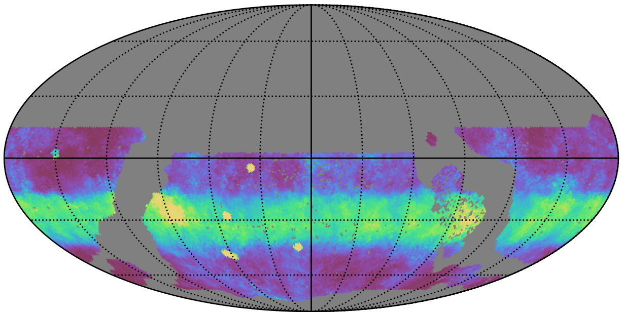
early_ss_template_fpextra2.0_v3.4_10yrs WFD y band: Median normairmass
