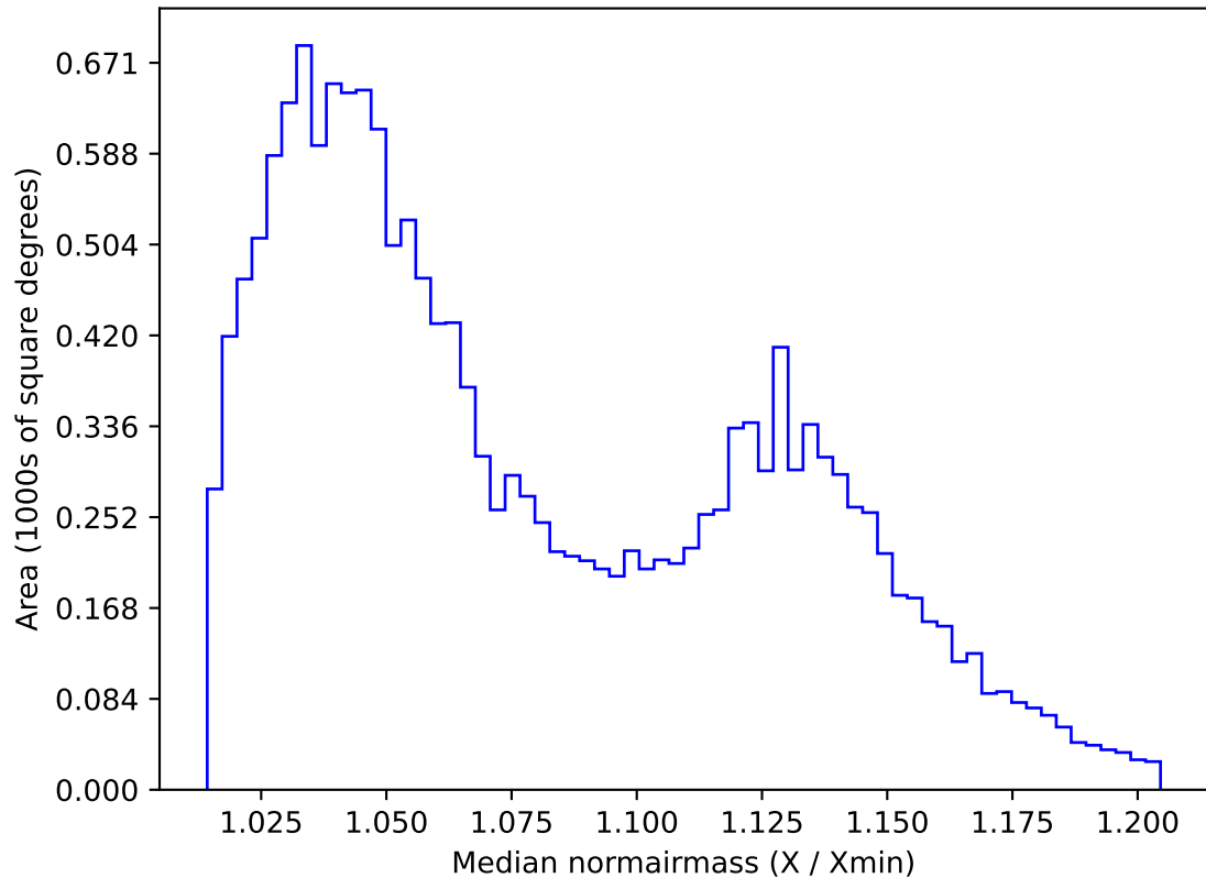
early_ss_template_fpextra2.0_v3.4_10yrs WFD g band: Median normairmass
