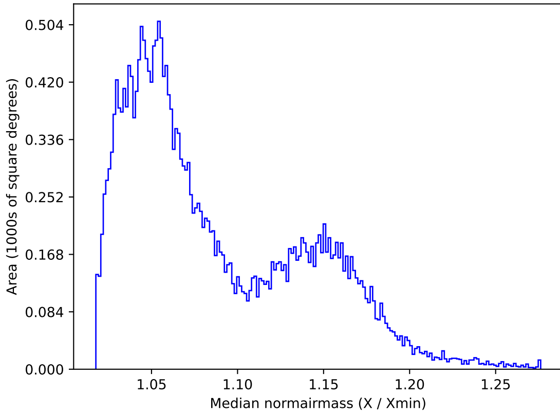
early_ss_template_fpextra2.0_v3.4_10yrs All sky z band: Median normairmass
