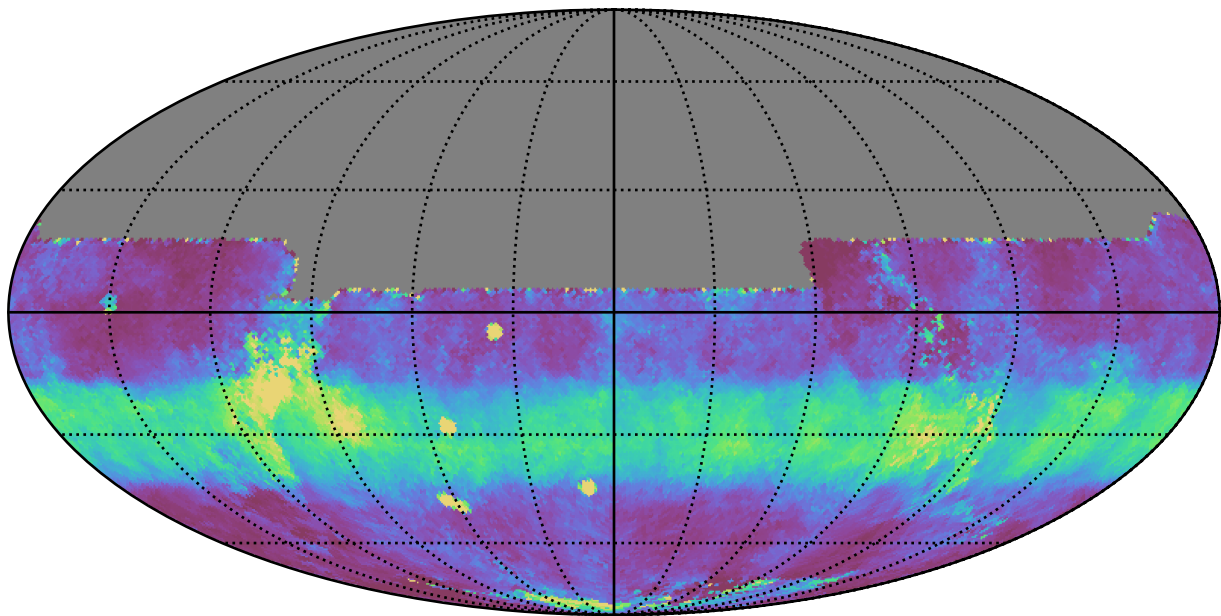
early_ss_template_fpextra2.0_v3.4_10yrs All sky y band: Median normairmass
