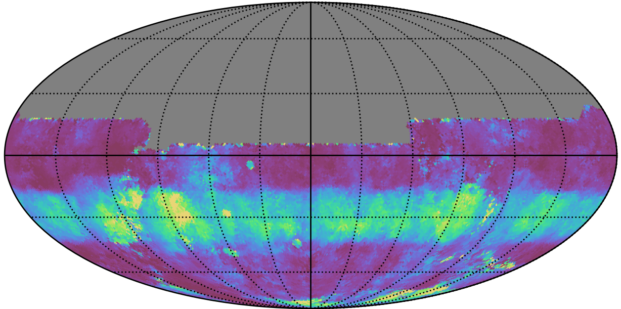
early_ss_template_fpextra2.0_v3.4_10yrs All sky u band: Median normairmass
