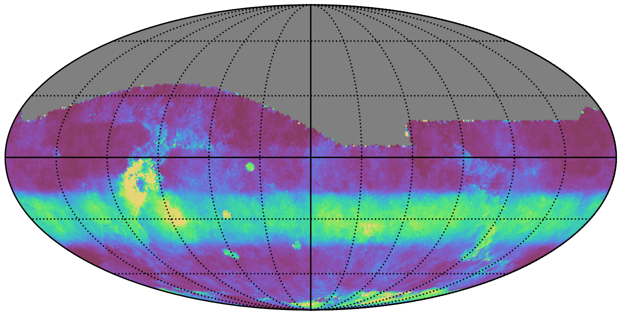
early_ss_template_fpextra2.0_v3.4_10yrs All sky i band: Median normairmass
