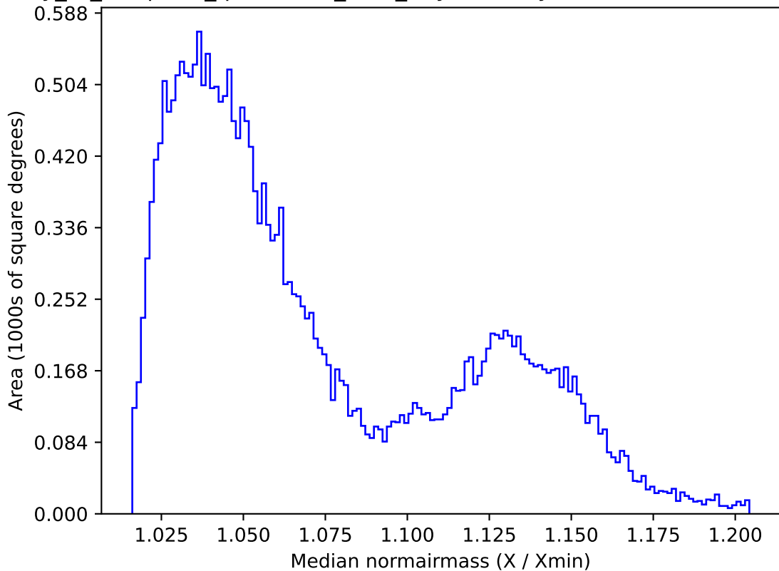
early_ss_template_fpextra2.0_v3.4_10yrs All sky i band: Median normairmass
