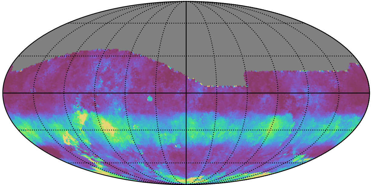
early_ss_template_fpextra2.0_v3.4_10yrs All sky g band: Median normairmass
