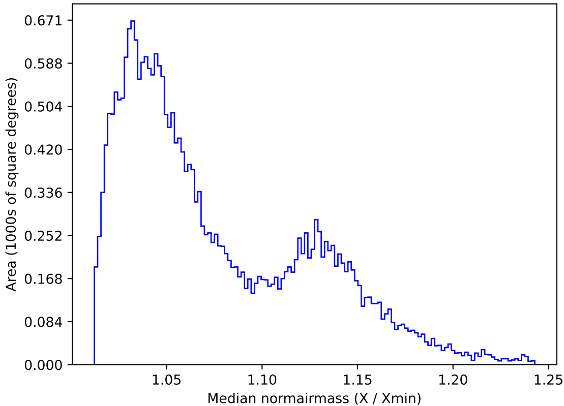
early_ss_template_fpextra2.0_v3.4_10yrs All sky g band: Median normairmass
