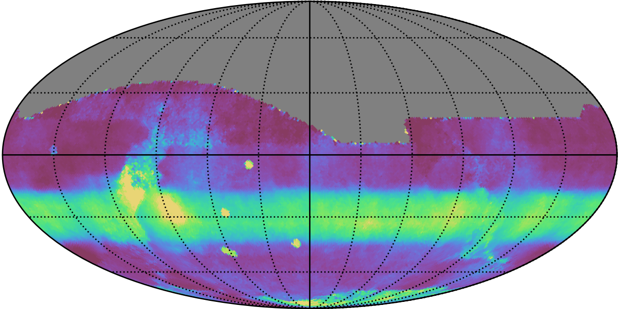
early_ss_template_fpextra2.0_v3.4_10yrs All sky all bands: Median normairmass
