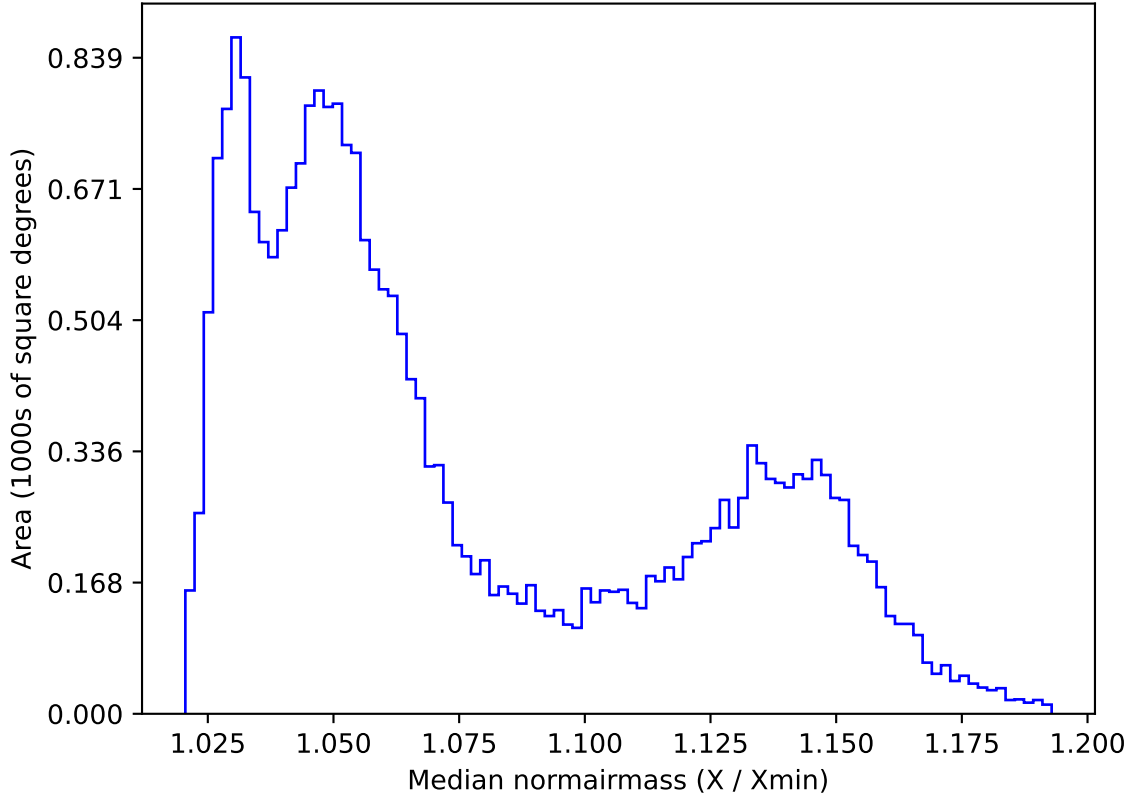
early_ss_template_fpextra2.0_v3.4_10yrs All sky all bands: Median normairmass
