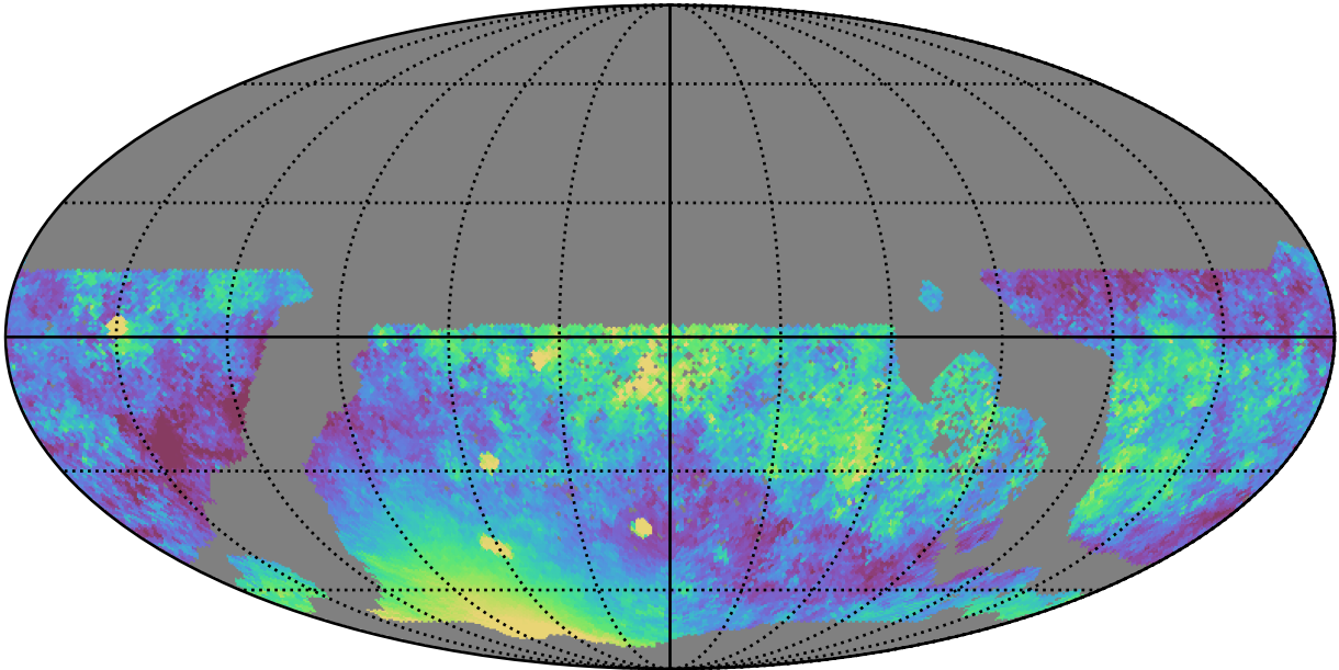
early_ss_template_fpextra2.0_v3.4_10yrs WFD z band: Median moonDistance
