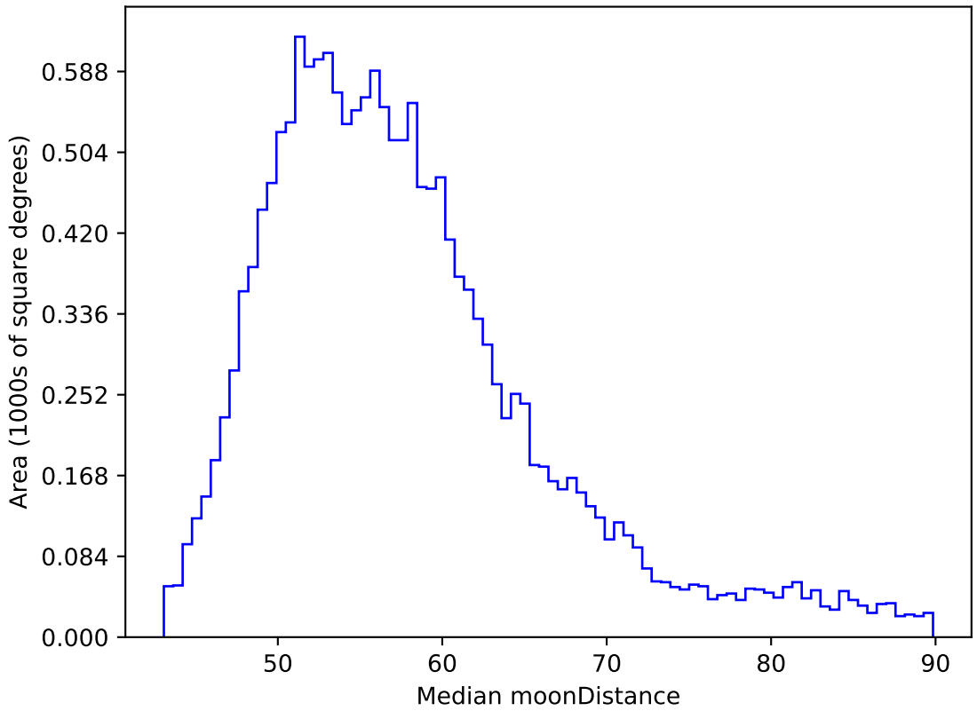
early_ss_template_fpextra2.0_v3.4_10yrs WFD y band: Median moonDistance
