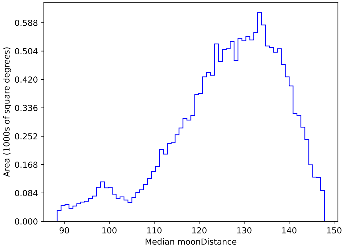
early_ss_template_fpextra2.0_v3.4_10yrs WFD u band: Median moonDistance
