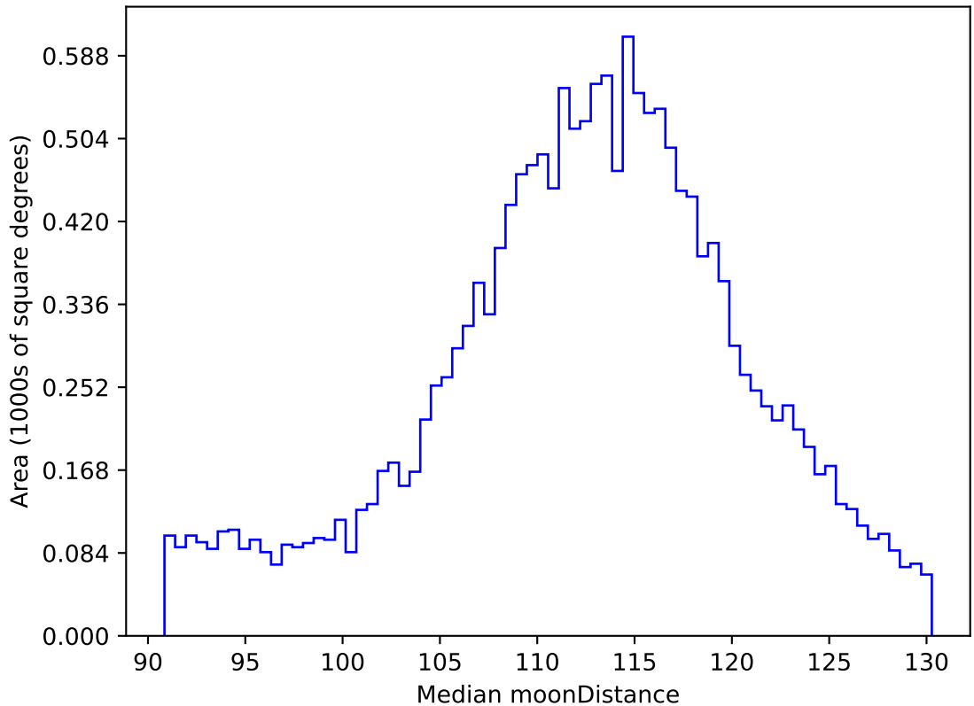
early_ss_template_fpextra2.0_v3.4_10yrs WFD r band: Median moonDistance
