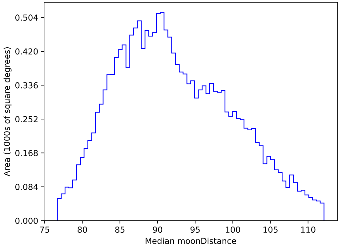
early_ss_template_fpextra2.0_v3.4_10yrs WFD i band: Median moonDistance
