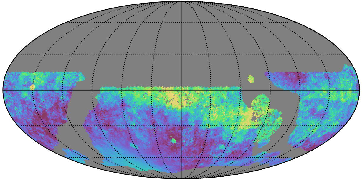
early_ss_template_fpextra2.0_v3.4_10yrs WFD all bands: Median moonDistance
