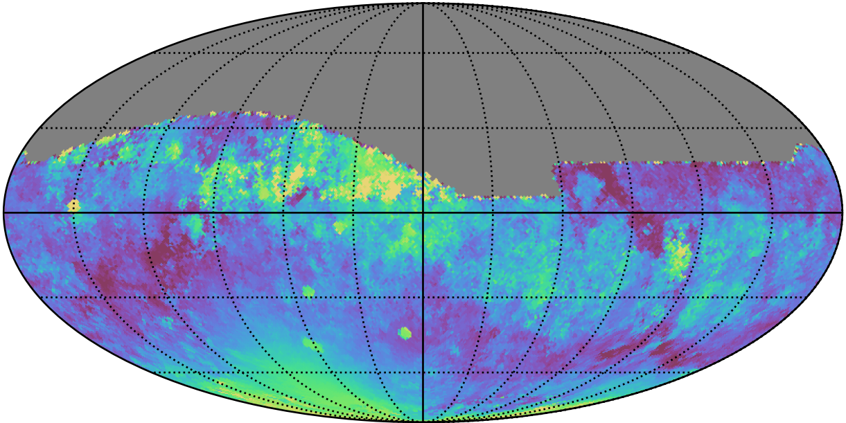
early_ss_template_fpextra2.0_v3.4_10yrs All sky z band: Median moonDistance
