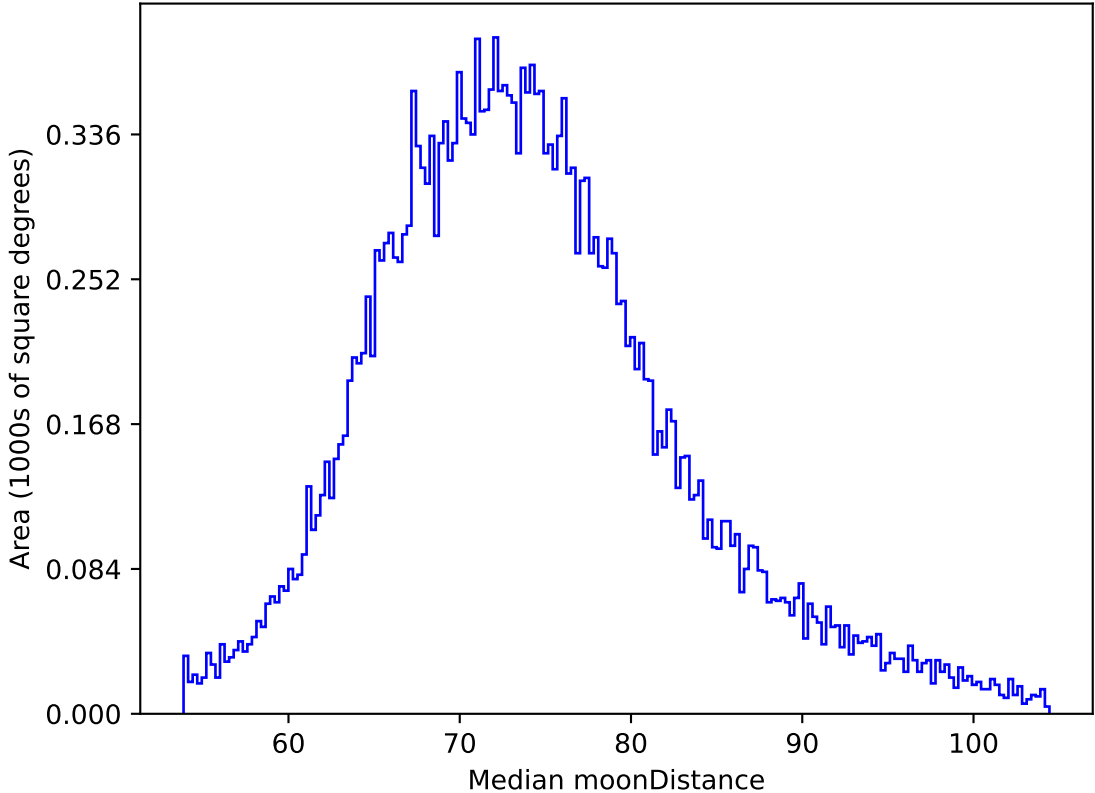
early_ss_template_fpextra2.0_v3.4_10yrs All sky z band: Median moonDistance
