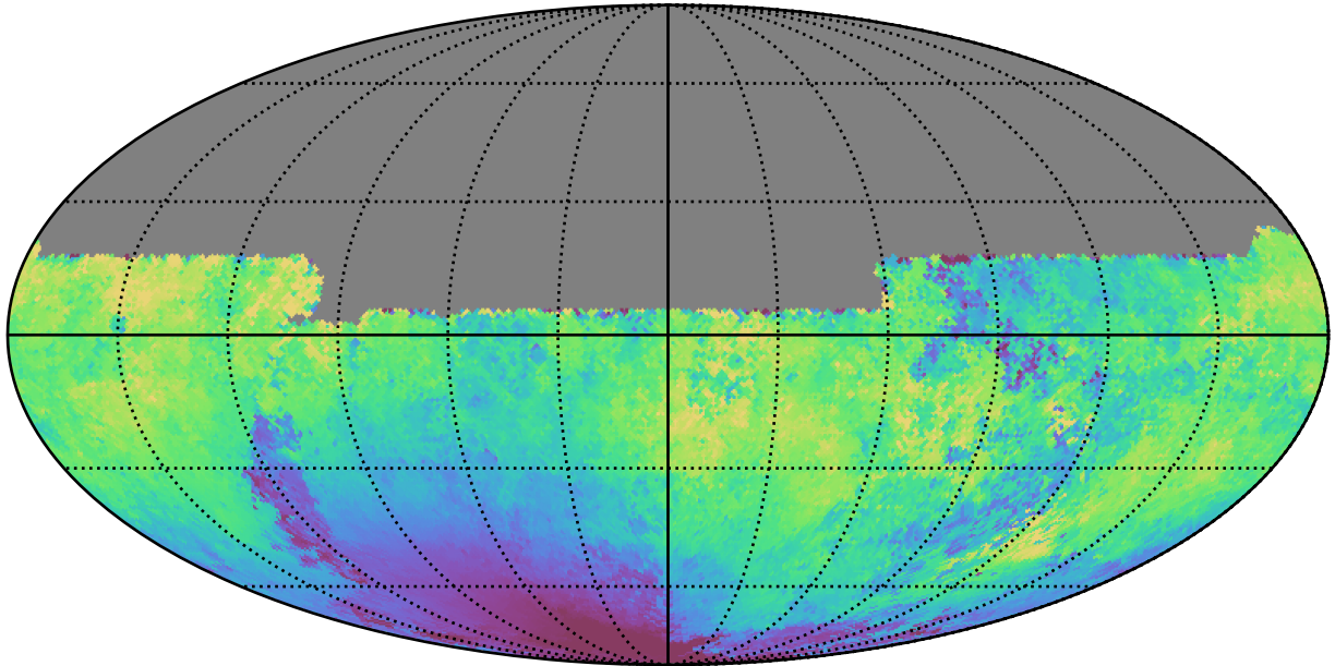
early_ss_template_fpextra2.0_v3.4_10yrs All sky u band: Median moonDistance
