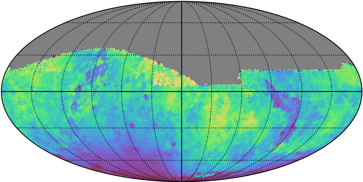
early_ss_template_fpextra2.0_v3.4_10yrs All sky r band: Median moonDistance
