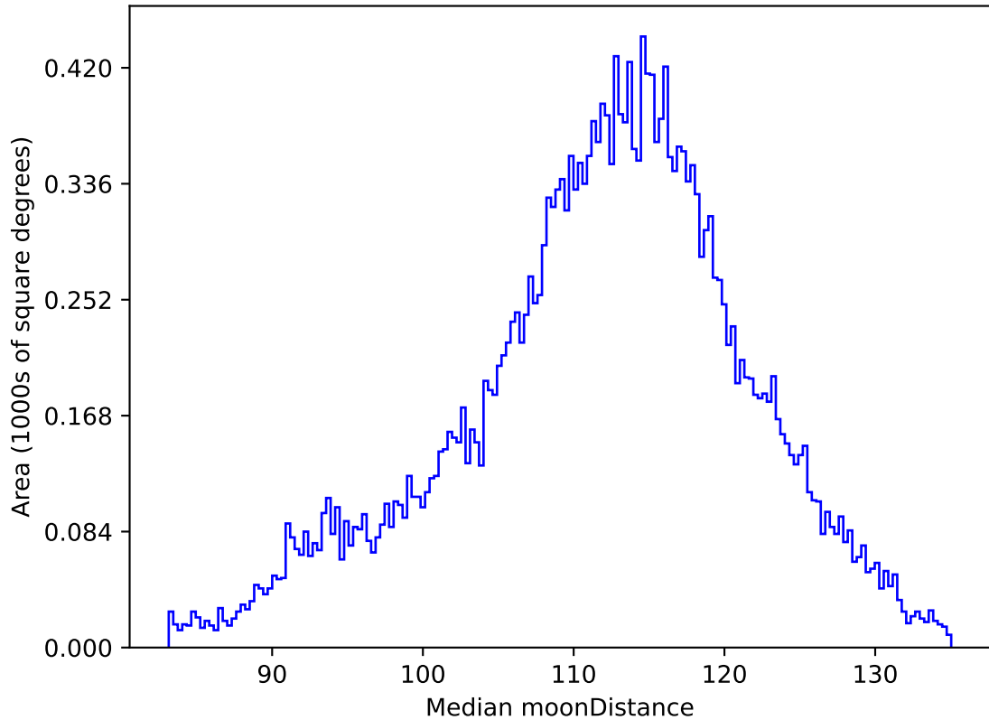
early_ss_template_fpextra2.0_v3.4_10yrs All sky r band: Median moonDistance
