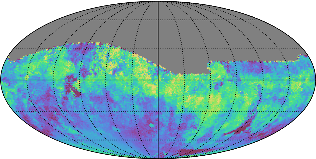
early_ss_template_fpextra2.0_v3.4_10yrs All sky i band: Median moonDistance
