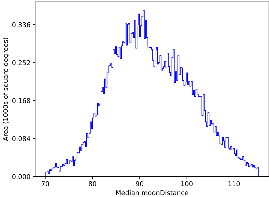
early_ss_template_fpextra2.0_v3.4_10yrs All sky i band: Median moonDistance
