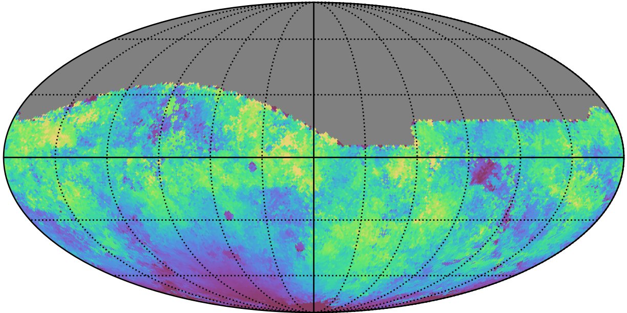
early_ss_template_fpextra2.0_v3.4_10yrs All sky g band: Median moonDistance
