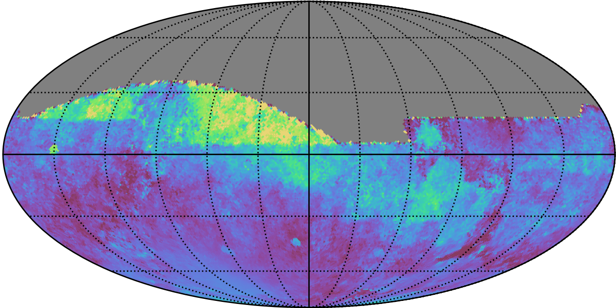
early_ss_template_fpextra2.0_v3.4_10yrs All sky all bands: Median moonDistance
