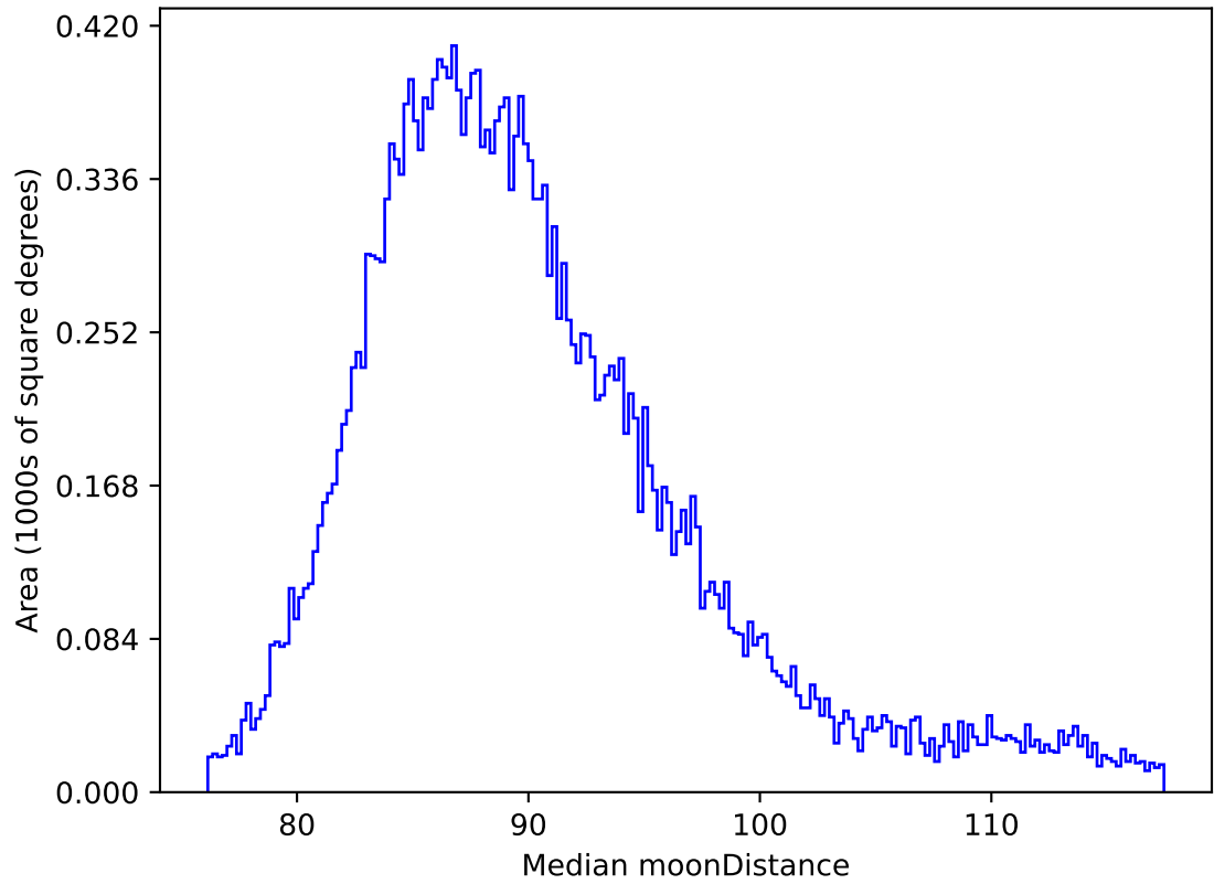
early_ss_template_fpextra2.0_v3.4_10yrs All sky all bands: Median moonDistance
