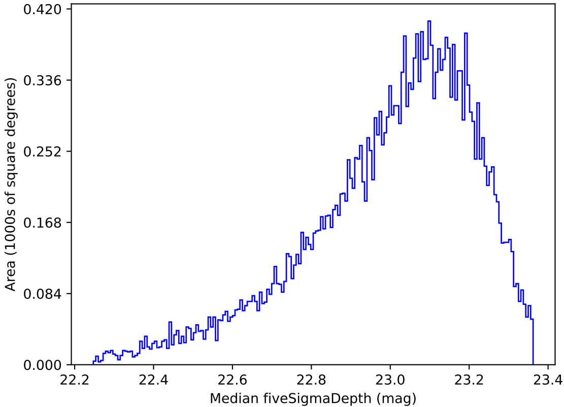
early_ss_template_fpextra2.0_v3.4_10yrs Yr 1 z band: Median fiveSigmaDepth
