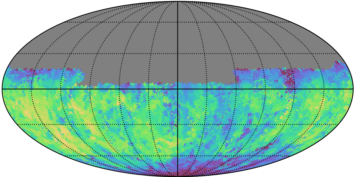
early_ss_template_fpextra2.0_v3.4_10yrs Yr 1 u band: Median fiveSigmaDepth
