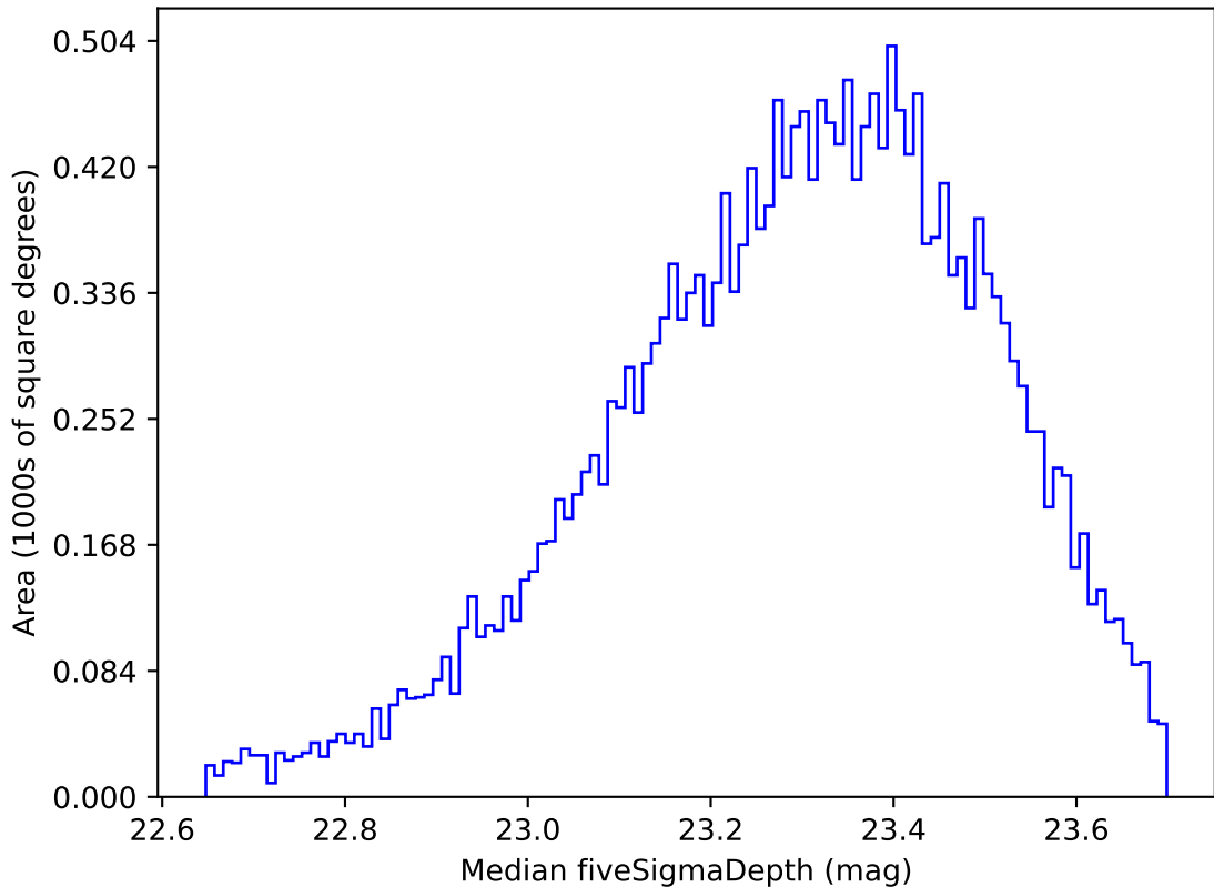
early_ss_template_fpextra2.0_v3.4_10yrs Yr 1 u band: Median fiveSigmaDepth
