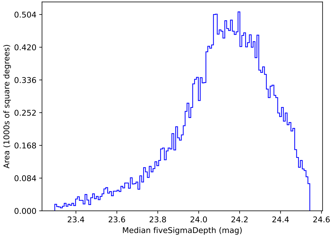
early_ss_template_fpextra2.0_v3.4_10yrs Yr 1 r band: Median fiveSigmaDepth
