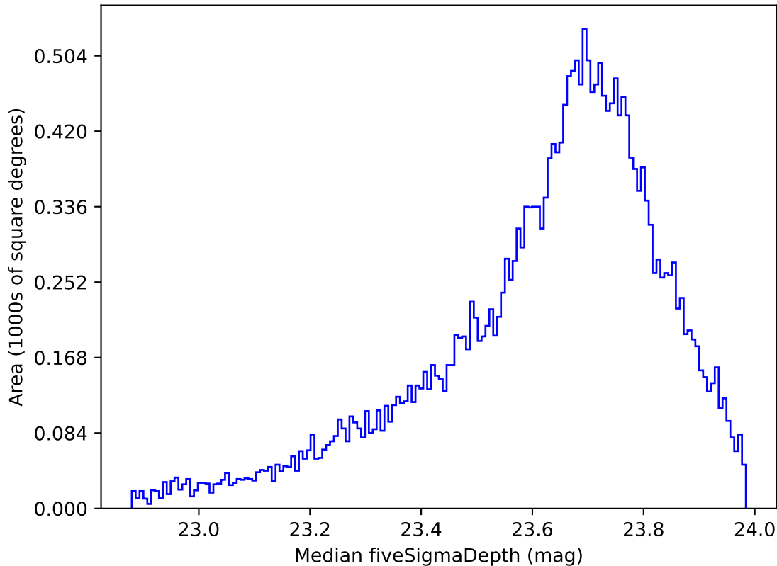
early_ss_template_fpextra2.0_v3.4_10yrs Yr 1 i band: Median fiveSigmaDepth
