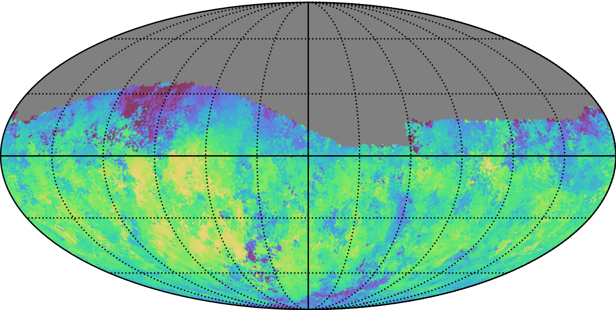
early_ss_template_fpextra2.0_v3.4_10yrs Yr 1 g band: Median fiveSigmaDepth
