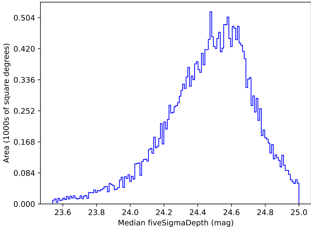
early_ss_template_fpextra2.0_v3.4_10yrs Yr 1 g band: Median fiveSigmaDepth
