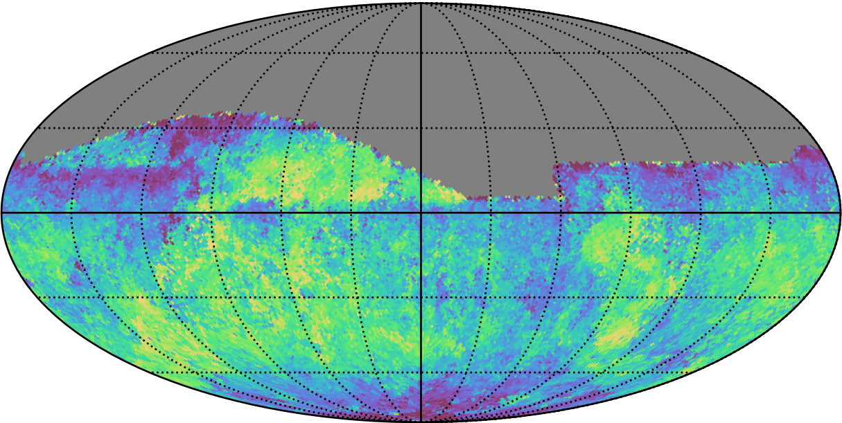
early_ss_template_fpextra2.0_v3.4_10yrs Yr 1 all bands: Median fiveSigmaDepth
