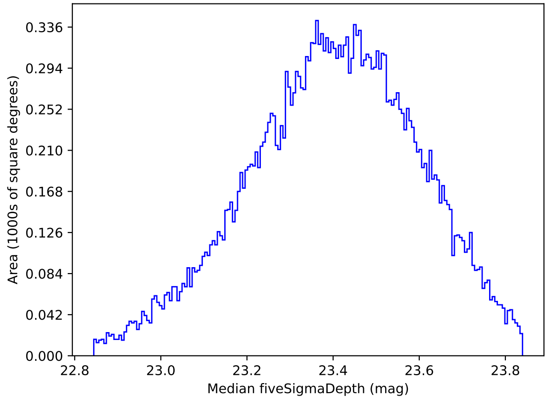
early_ss_template_fpextra2.0_v3.4_10yrs Yr 1 all bands: Median fiveSigmaDepth
