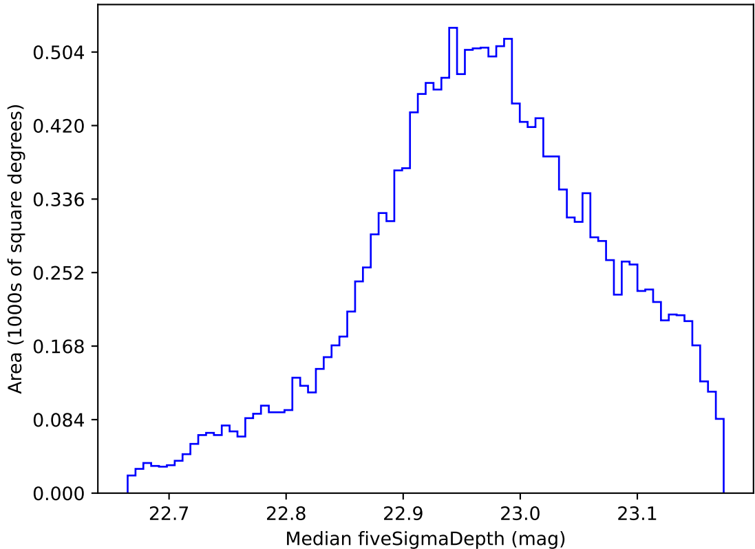
early_ss_template_fpextra2.0_v3.4_10yrs WFD z band: Median fiveSigmaDepth
