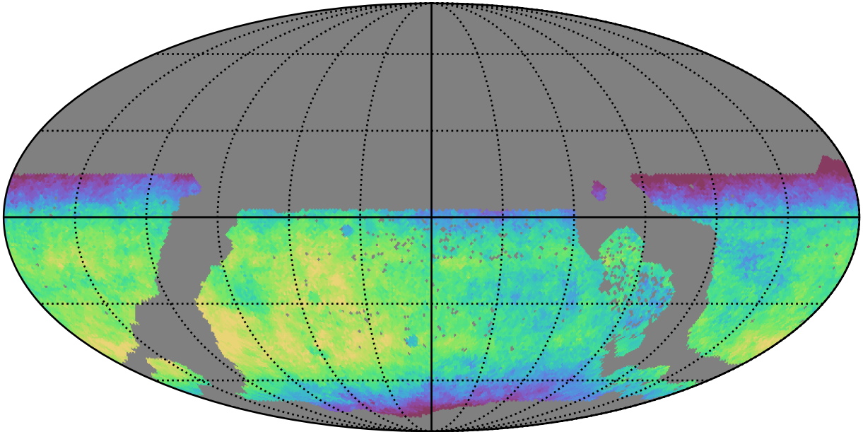
early_ss_template_fpextra2.0_v3.4_10yrs WFD y band: Median fiveSigmaDepth
