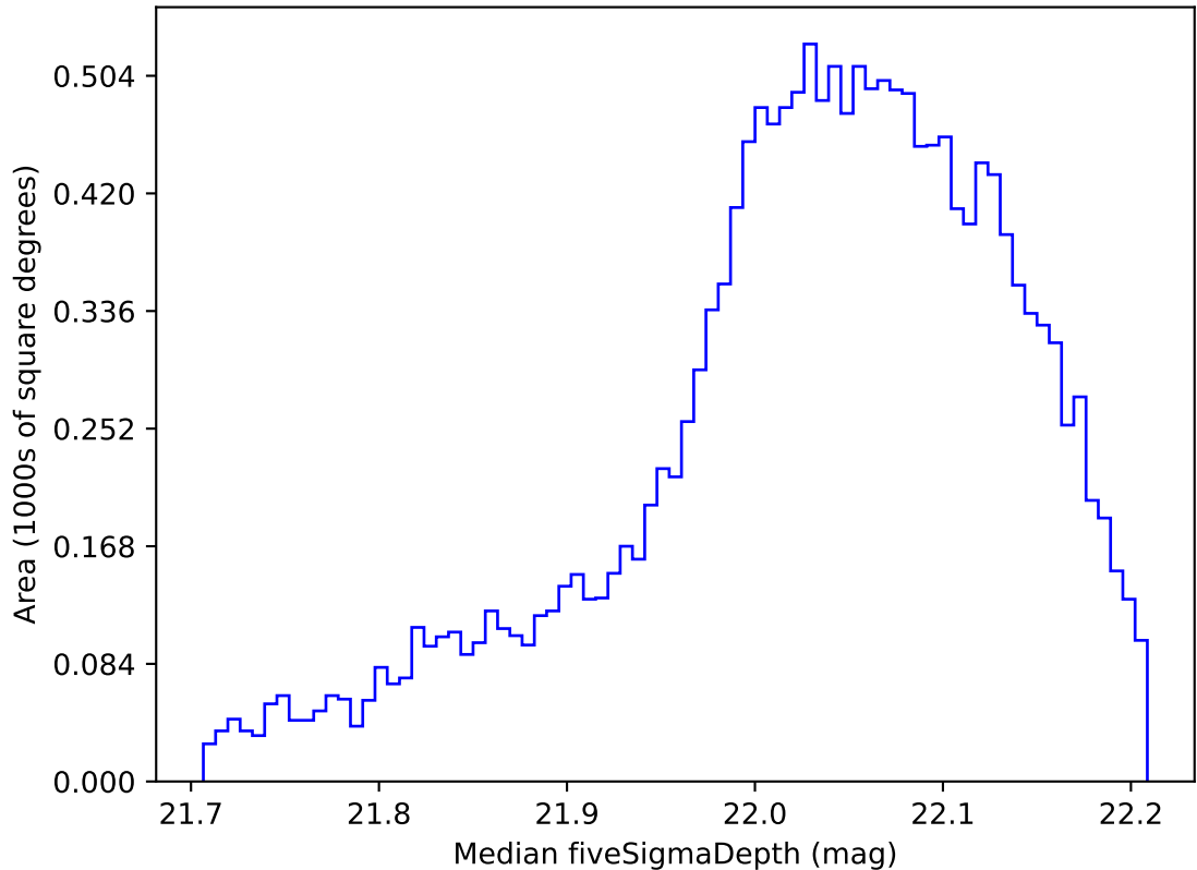
early_ss_template_fpextra2.0_v3.4_10yrs WFD y band: Median fiveSigmaDepth
