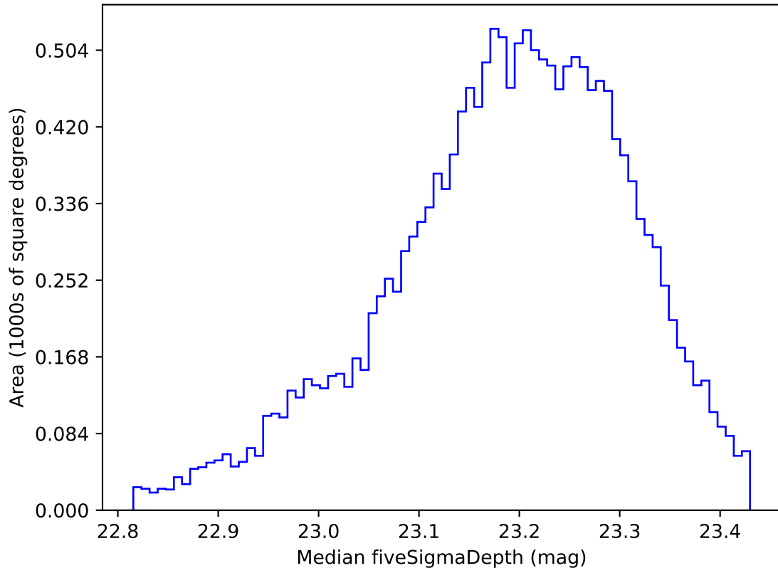
early_ss_template_fpextra2.0_v3.4_10yrs WFD u band: Median fiveSigmaDepth
