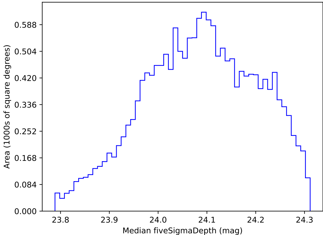
early_ss_template_fpextra2.0_v3.4_10yrs WFD r band: Median fiveSigmaDepth
