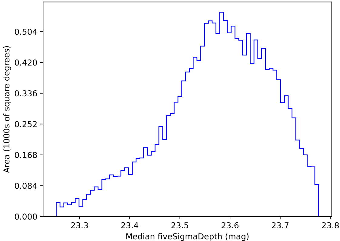
early_ss_template_fpextra2.0_v3.4_10yrs WFD i band: Median fiveSigmaDepth
