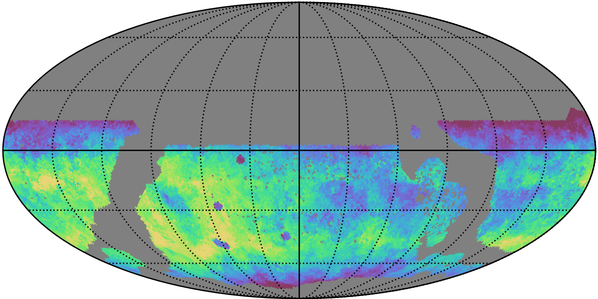
early_ss_template_fpextra2.0_v3.4_10yrs WFD g band: Median fiveSigmaDepth
