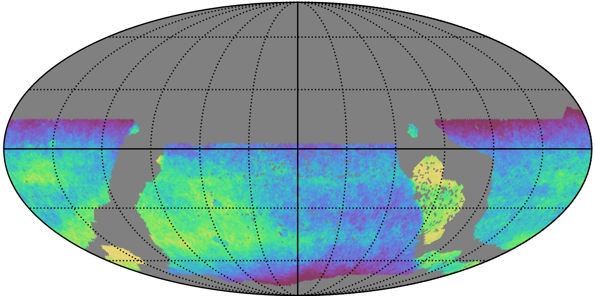
early_ss_template_fpextra2.0_v3.4_10yrs WFD all bands: Median fiveSigmaDepth
