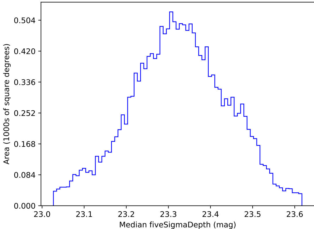
early_ss_template_fpextra2.0_v3.4_10yrs WFD all bands: Median fiveSigmaDepth
