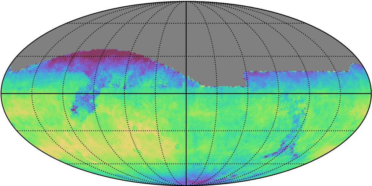
early_ss_template_fpextra2.0_v3.4_10yrs All sky z band: Median fiveSigmaDepth
