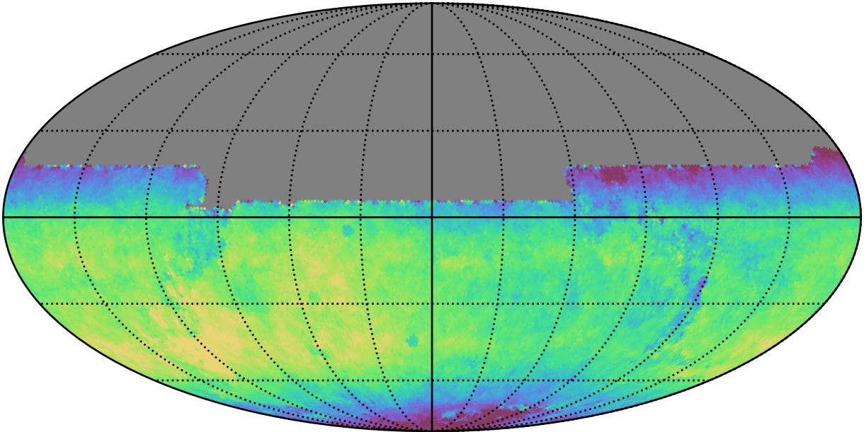
early_ss_template_fpextra2.0_v3.4_10yrs All sky y band: Median fiveSigmaDepth
