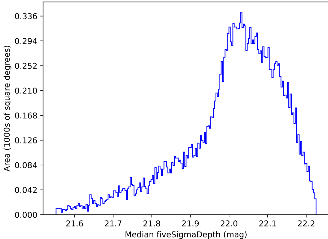
early_ss_template_fpextra2.0_v3.4_10yrs All sky y band: Median fiveSigmaDepth
